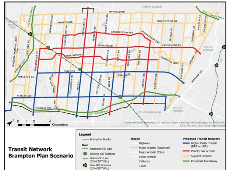
Figure 3-2: 2051 Network Maps for Brampton Plan Scenario
