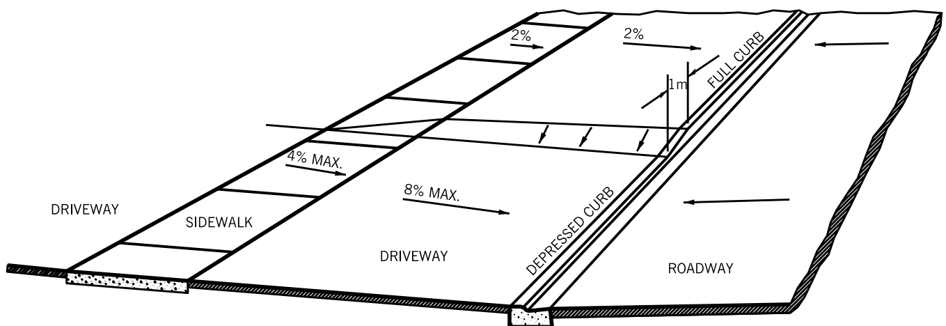
ISOMETRIC VIEW
