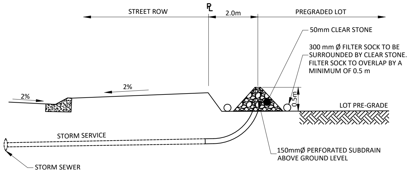
CROSS SECTION
