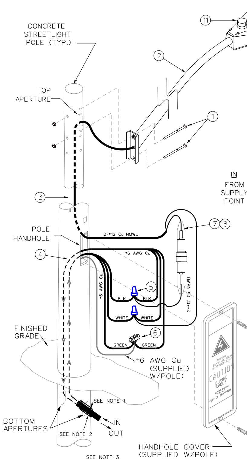
SCHEMATIC DIAGRAM
