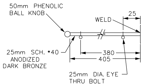
POLE PLATE AND ARM DETAILS
