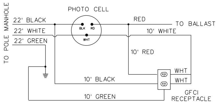
SCHEMATIC DIAGRAM
